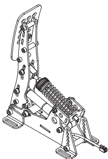
THROTTLE
